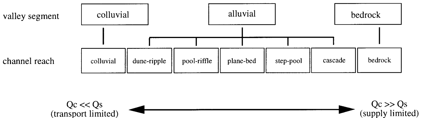
Figure 11. Schematic illustration of the transport capacities relative to sediment supply for reach-level channel types.
