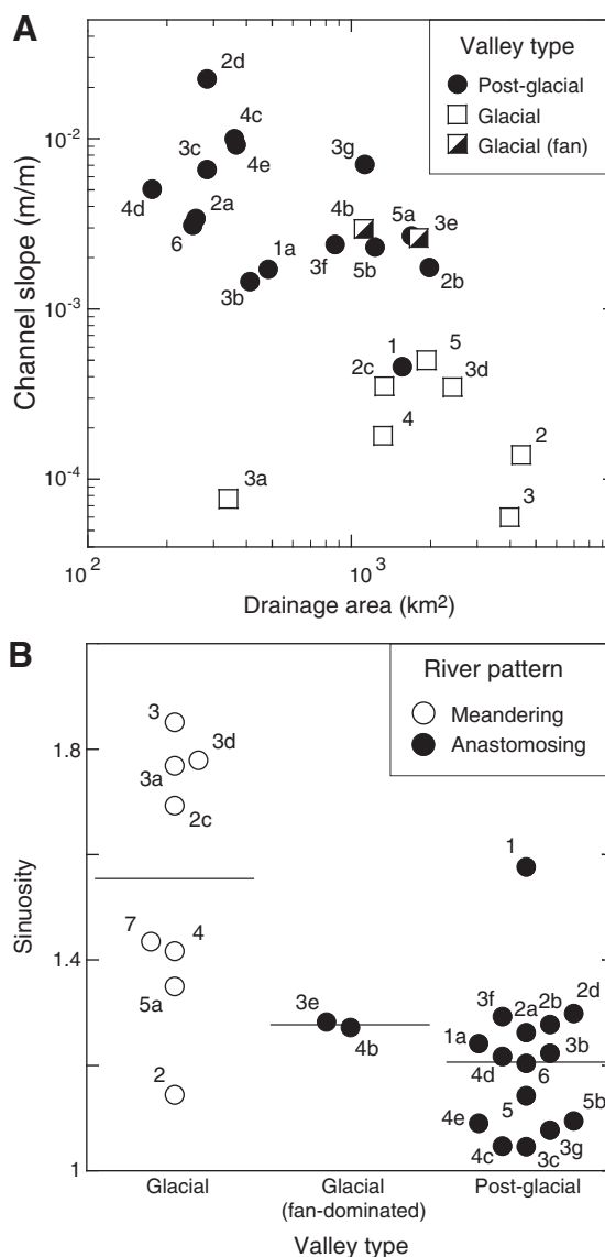
Fig. 8. (A) Drainage area, channel slope, and channel pattern for valley segments identified in Fig. 1 and Table 1. Solid circles are post-glacial valleys; open squares are glacial valleys; half-filled squares are fan-dominated glacial valley segments. (B) Sinuosity measured from reconstructed historical river channels (from Table 1), for glacial, fan-dominated glacial, and post-glacial valleys. Horizontal line is mean for each group. Mean and standard error: glacial valleys = 1.55 \pm 0.09 ; fan-dominated glacial valleys = 1.28 \pm 0.005 ; post-glacial valleys = 1.21 \pm 0.04 .
