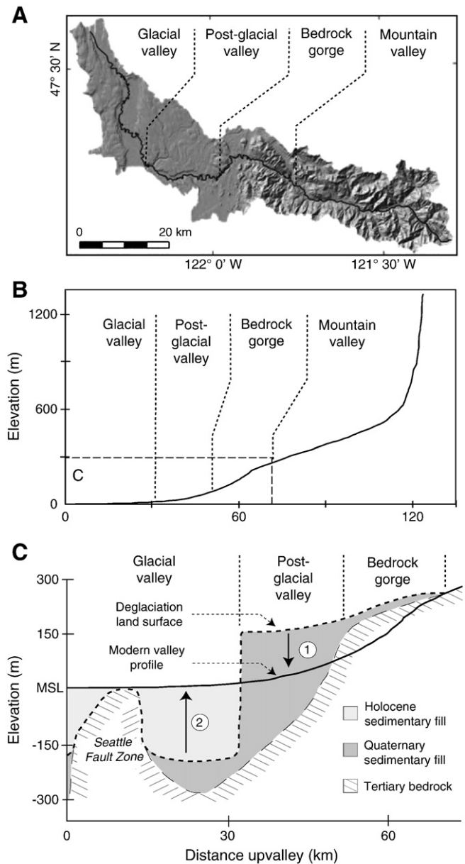
Fig. 2. Schematic longitudinal valley profile of the Duwamish–Green River showing glacial and post-glacial valleys. Schematic shows Pleistocene valley fill above bedrock, original post-glacial surface of glacial trough, and (1) Holocene degradation into lowland fill and (2) Holocene aggradation into glacial trough.
